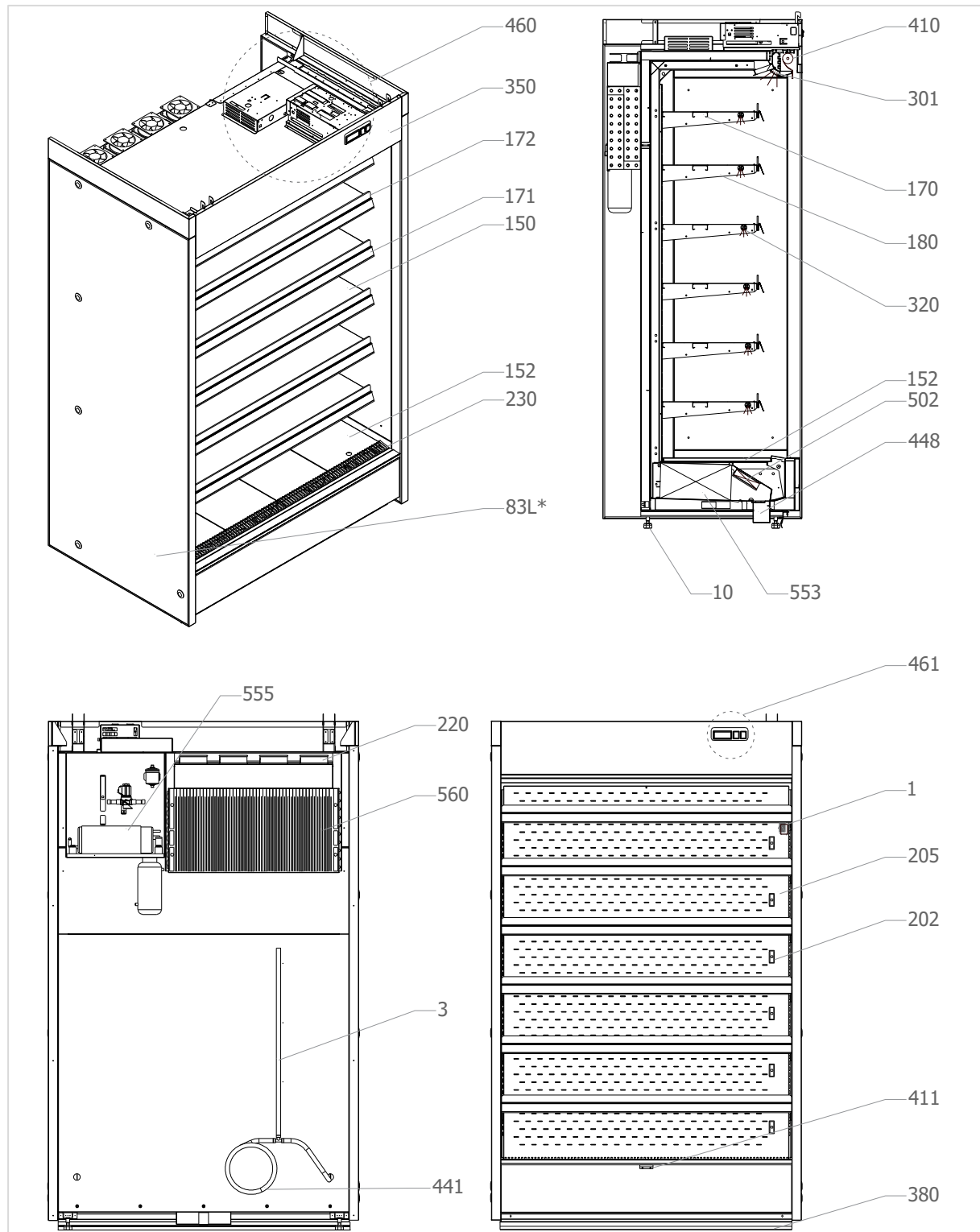
Figure 1 KING EVO_King 2 – PLUG IN version - device construction
