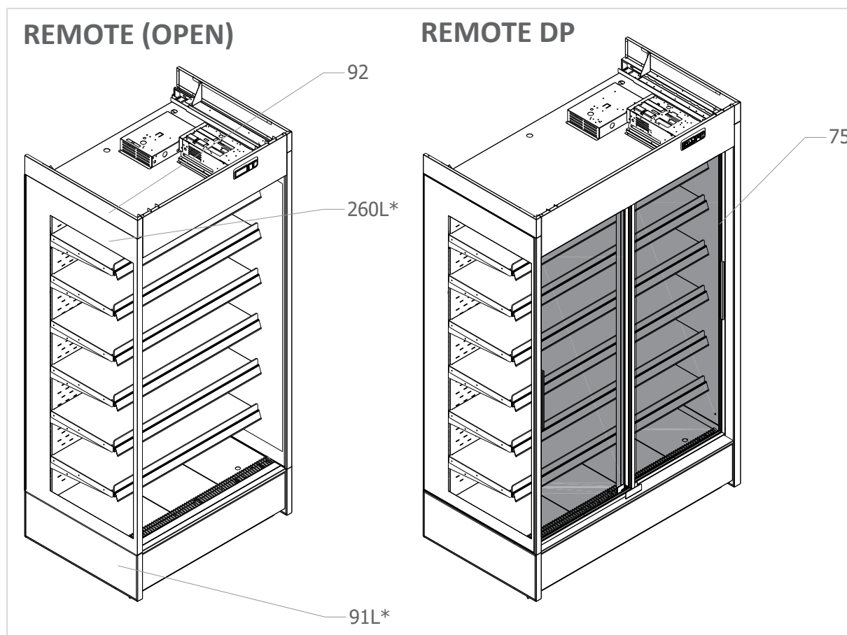
Figure 2 KING EVO_King 2 – REMOTE version - differences in device construction
