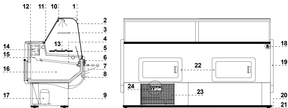
Fig.1 Construction of the device
