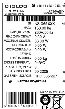
Fig.12 Data plate
